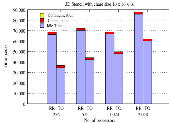
Fig. 4. Effect of topology mapping on latency on Blue Gene/L (RR: Round-Robin, TO: Topology, Data Size: 512 \times 512 \times 512 )
