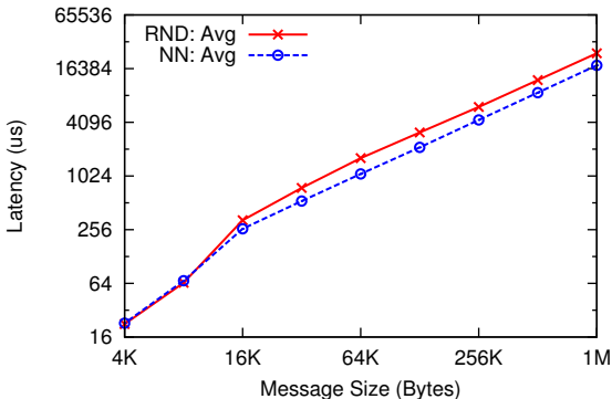
Latency vs. Msg Size: With Contention (8K cores, Ranger)
