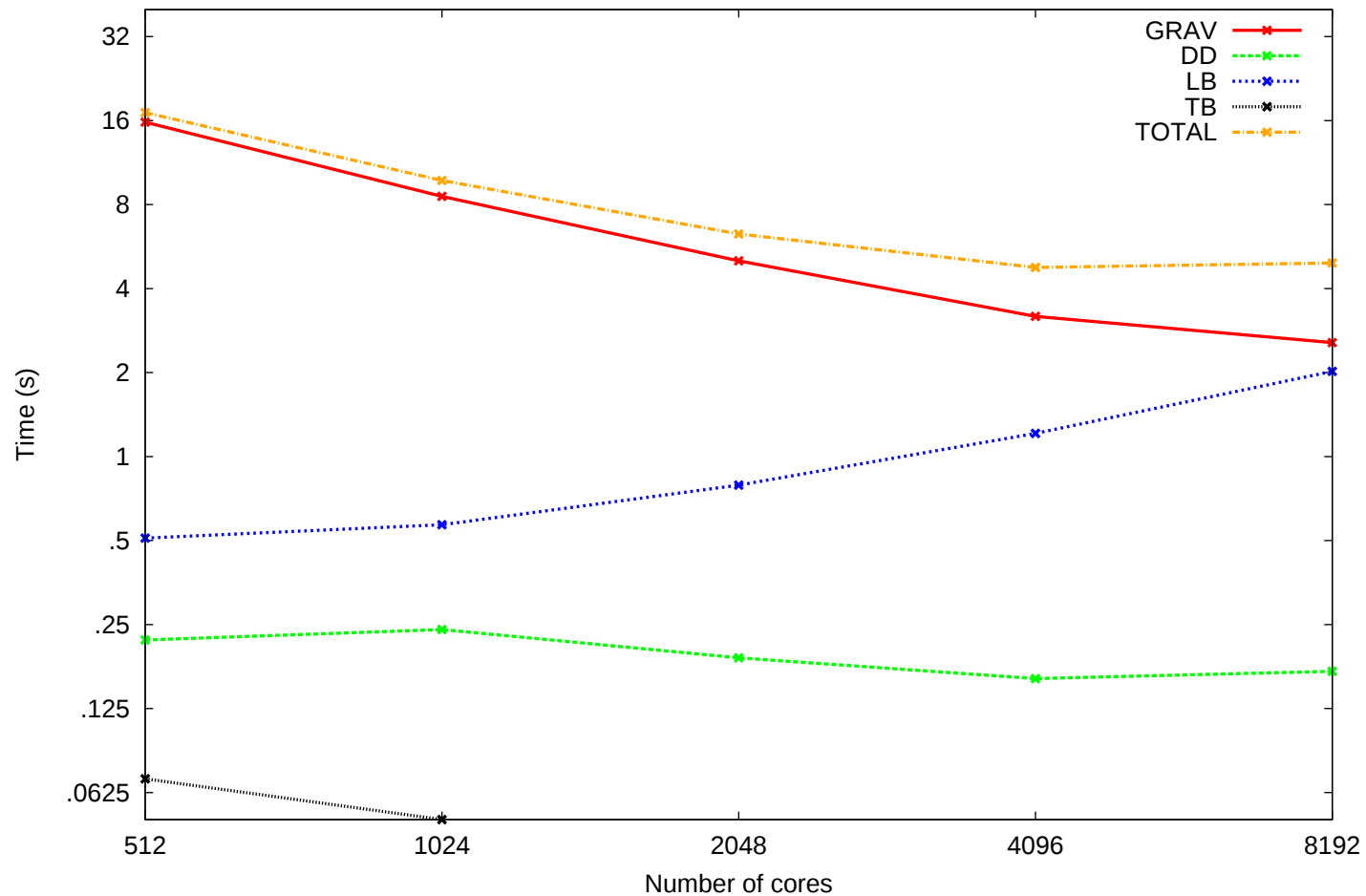
Breakdown of ChaNGa execution time for cosmo50 (Single stepping)
