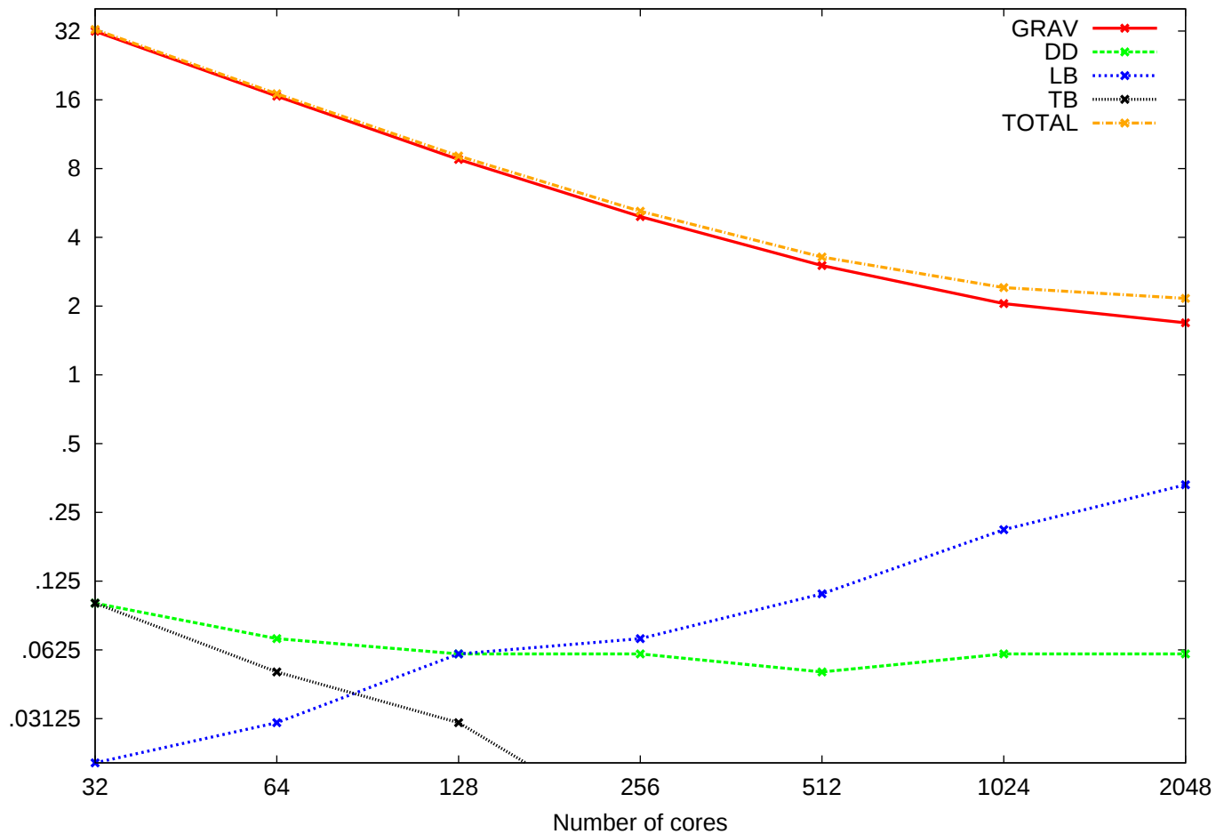
Breakdown of ChaNGa execution time for HRWH (Single stepping)
