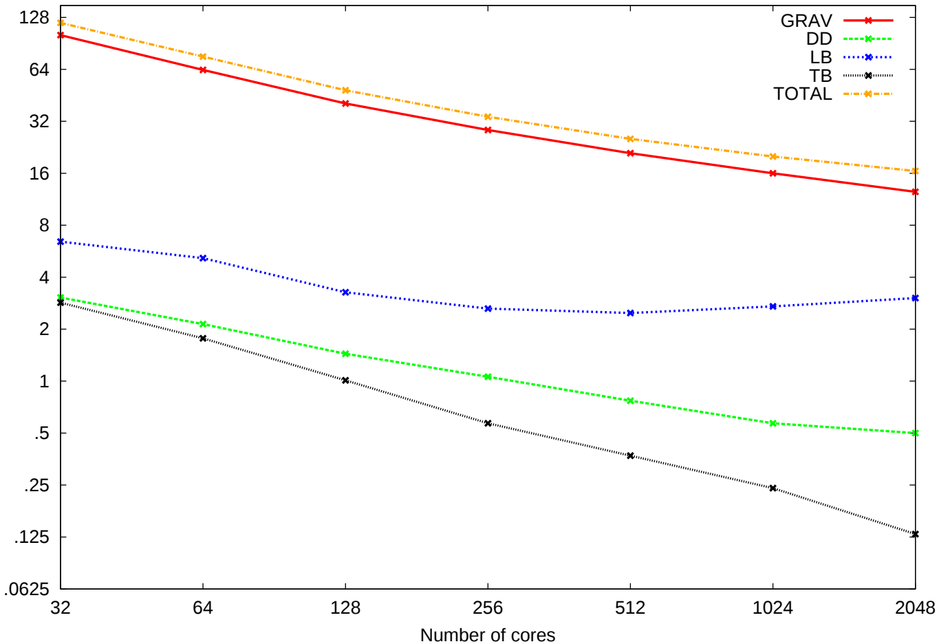
Breakdown of ChaNGa execution time for HRWH (Multisteping)
