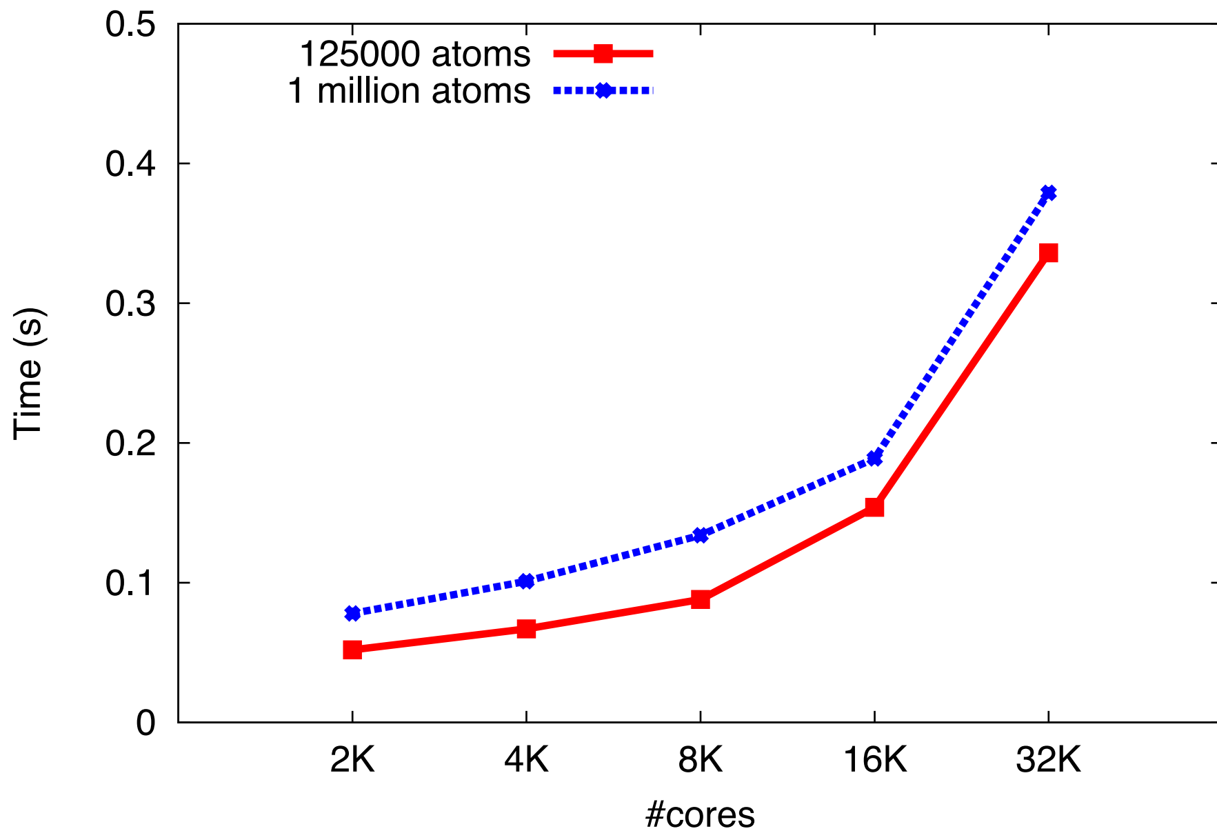
Restart Time – Intrepid(leanMD)
