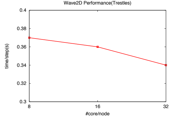
Figure 2.4: Performance improvement using more cores on each node
