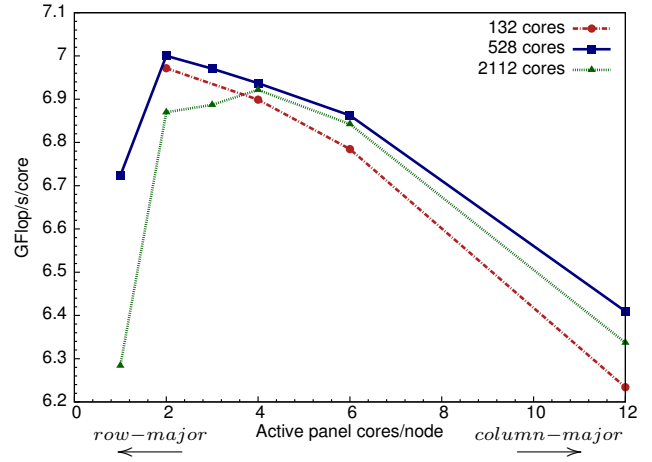
Fig. 9. Performance effects of striding the block-cyclic mapping with rotation and a tall process grid. 1 PE per node is effectively row-major (stride = process grid width), while 12 PEs per node is effectively column major (stride = 1). Results are from weak scaling on XT5.
