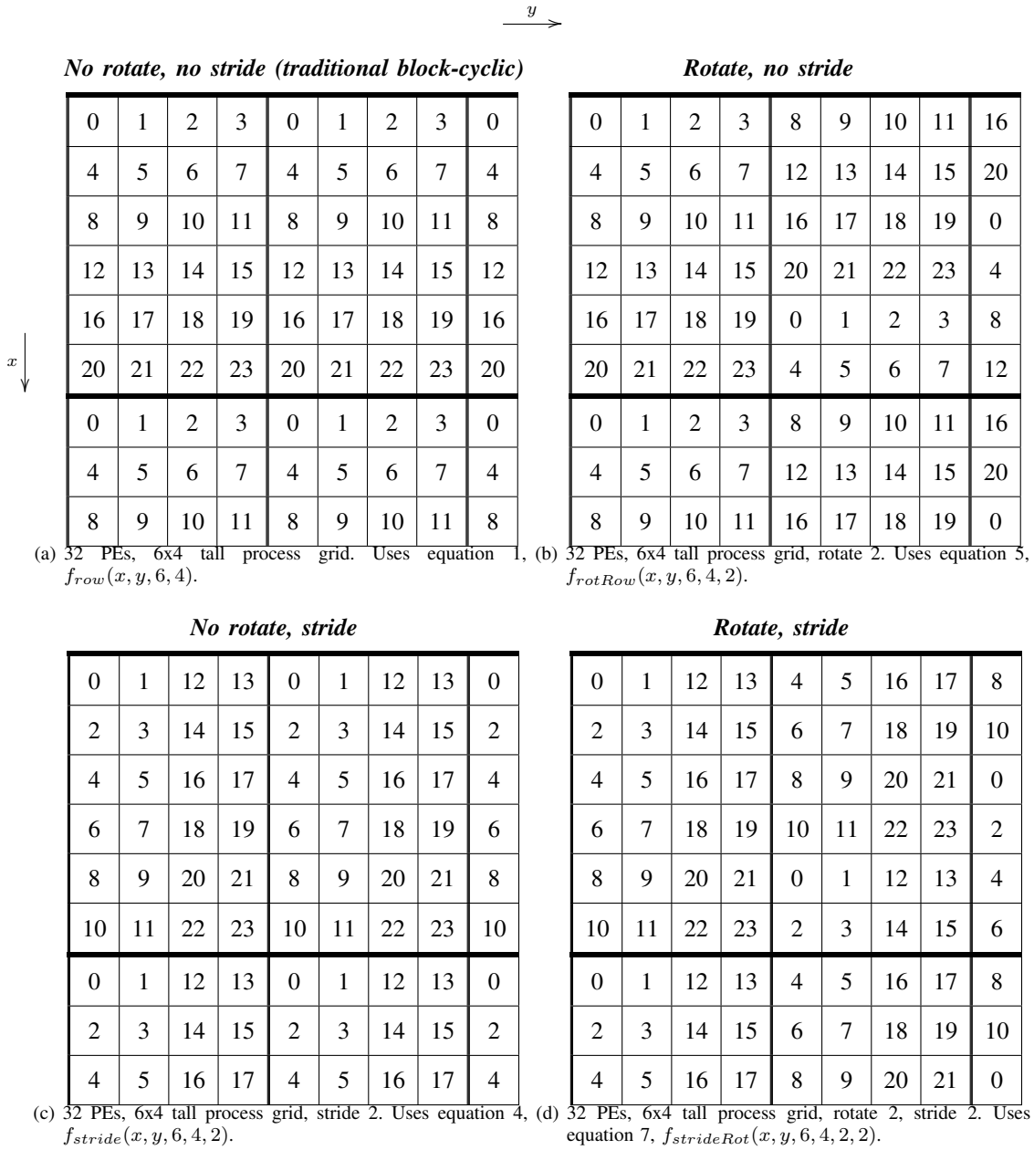
Fig. 1. Block-cyclic mapping scheme using a tall process grid and applying rotation and striding to increase performance. Rotation increases the amount of row parallelism and striding increases active panel locality.
