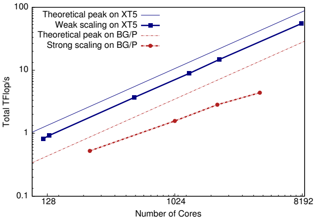
Fig. 10. Weak scaling (memory usage of matrix is constant around 75%) from 120 to 8064 processors on Jaguar, a Cray XT5 machine with 12 cores per node. Strong scaling ( n = 96,000 ) from 256 to 4096 processors on Intrepid, an IBM BG/P machine with 4 cores per node.
