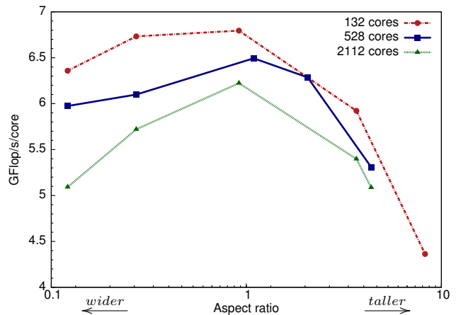
Fig. 7. Various aspect ratios for the process grid of a row-major block-cyclic distribution. Approximately square process grids perform the best. Tall process grids decrease performance because they lack parallelism in U. Wide process grids decrease performance because they slow down the active panel. Results are from weak scaling on XT5.
