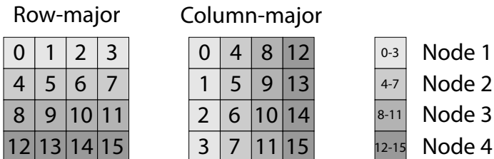
Fig. 3. Row-major and column-major process grid configurations with 4-core node.
