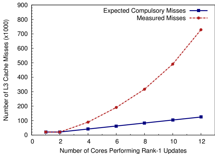
Fig. 4. Number of L3 cache misses on a node of Jaguar (dual Istanbul processors), as increasing numbers of cores are used to perform rank-1 updates
