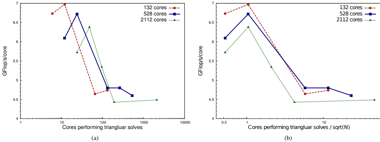
Fig. 8. The effect of adding rotation to a tall process grid to gain the benefits of a fast panel factorization, which is provided by the tall grid, and row parallelism which is recovered by rotating the process grid in the x direction. The same data is graphed in (b), but with the x -axis scaled by \sqrt{\#\text{cores}} to illustrate that the ideal U parallelism matches the amount given by a square process grid. Results are from weak scaling on XT5.
