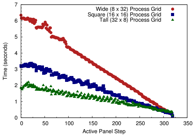
Fig. 6. The time to factorize each panel of matrix blocks for wide, square, and tall process grids. The tall process grid reduces the time due to increased exploitation of computational parallelism along the column of the process grid. Experiments were performed on BG/P on 256 cores using a 96000 \times 96000 matrix with a block size of 300 \times 300 in a row-major configuration.
